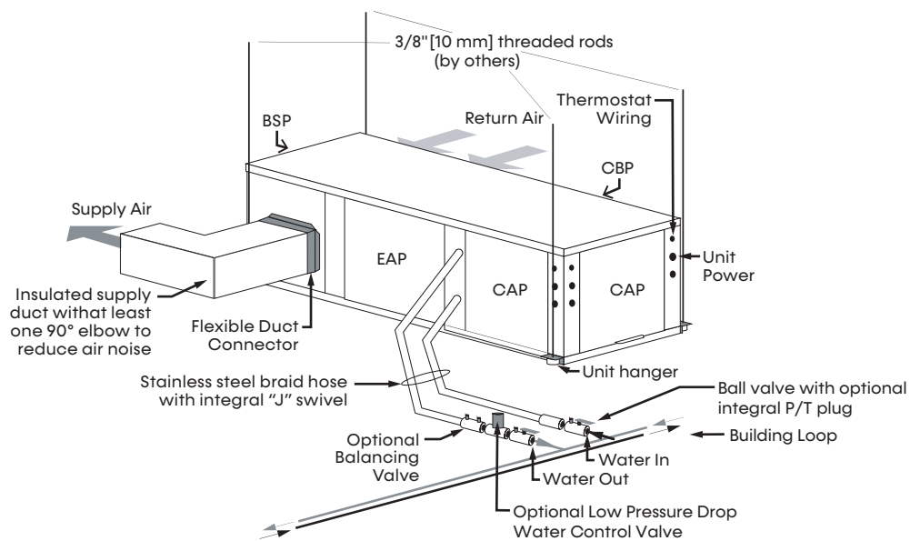
Figure 9: Typical Water-Loop Application
