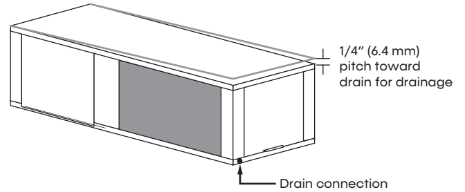
Figure 2: Horizontal Unit Pitch
