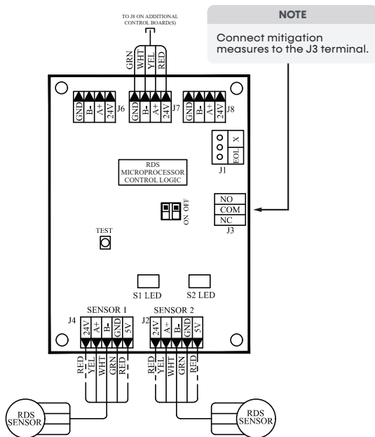
Figure 19: RDS Board
