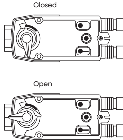
Figure 11: Internal Modulating Motorized Valve Positions
