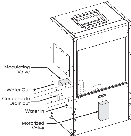
Figure 10: Typical Closed-Loop with Central-Pumping Application
