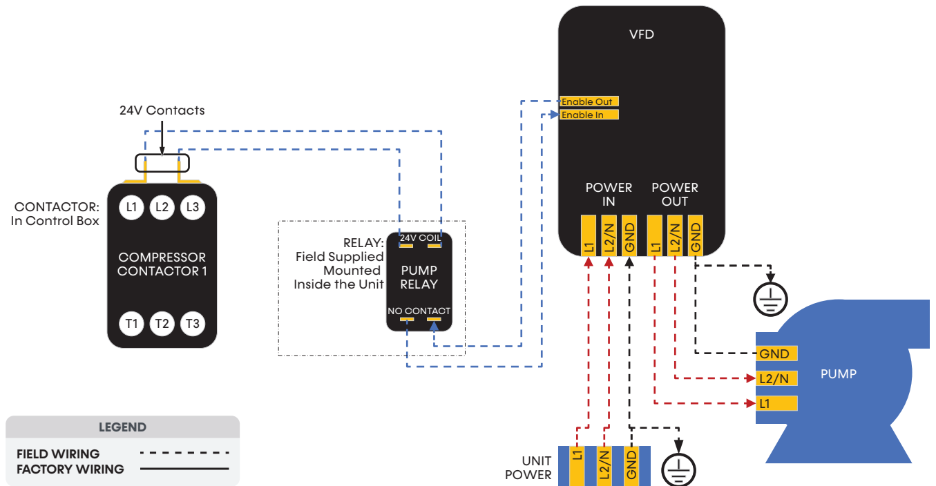
Figure 18: External Pump Control with VFD Diagram
