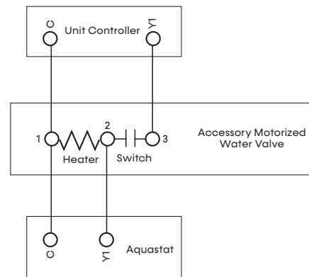
Figure 15: Optional Motorized Water Valve Wiring
