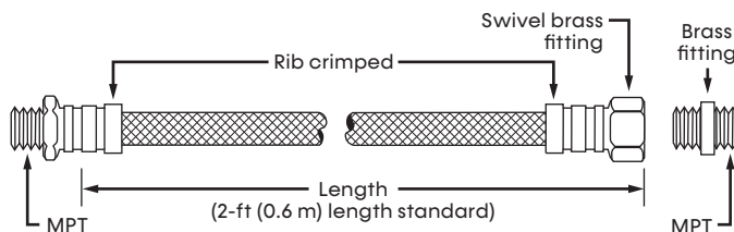
Figure 8: Supply/Return Hose Kit
