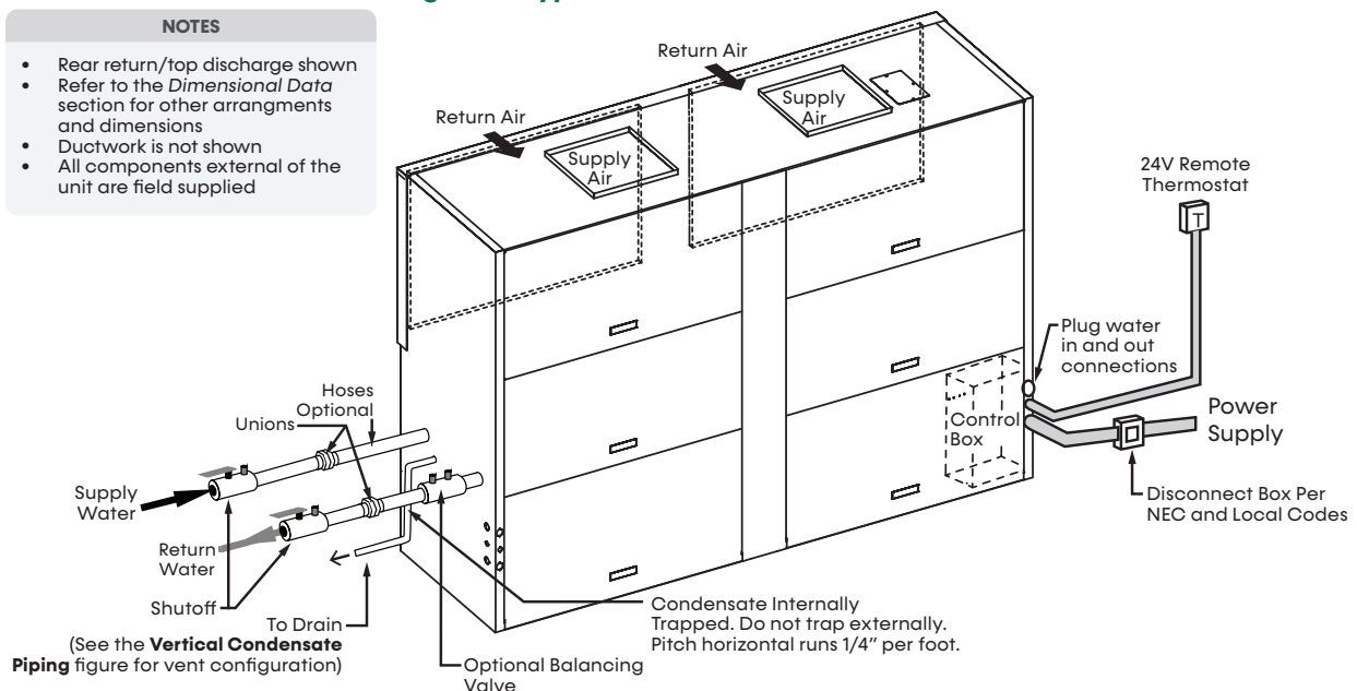
Figure 6: Typical Vertical Unit Installation
