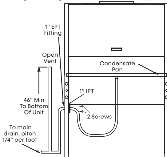
Figure 7: Vertical Condensate Piping All fittings and tubing outside of the unit are field supplied.
