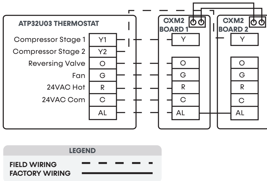
Figure 16: Thermostat Connection
