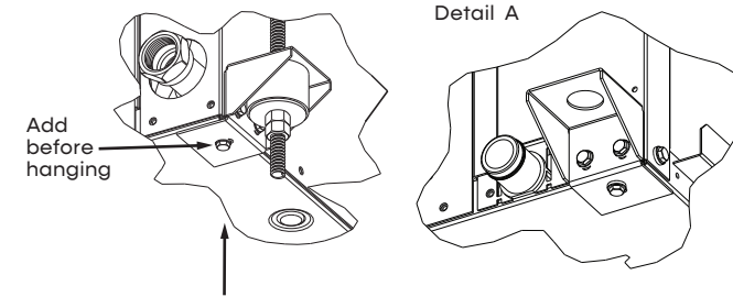
Figure 1: Hanger Bracket
