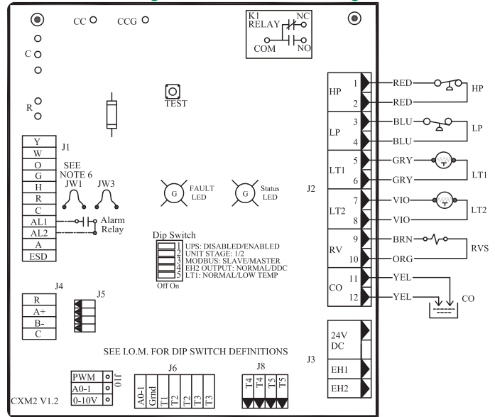
Figure 12: LT1 Limit Setting
