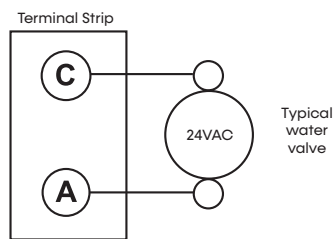
Figure 14: Accessory Wiring
