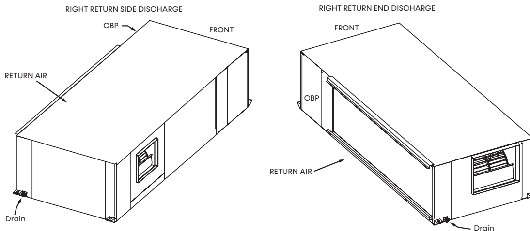
Figure 5: Right Return Side Discharge to Back
