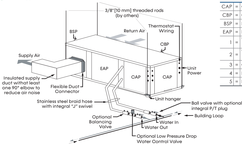
Figure 3: Typical Horizontal Unit Installation
