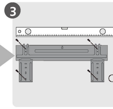
Fixez la plaque support
