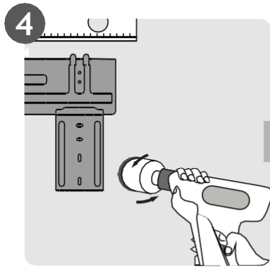
Perforar la pared
