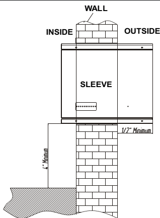
SLEEVE INSTALLATION
