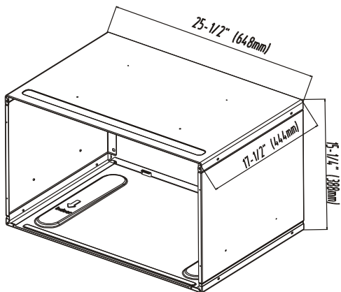
SLEEVE DIMENSION
