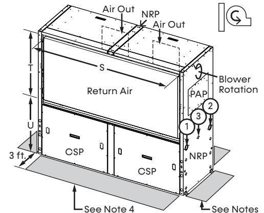
Blower to Air Coil relationship for Straight Discharge sizes 168-240
