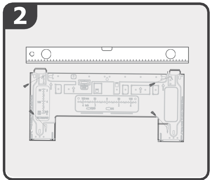
Fixez la plaque support
